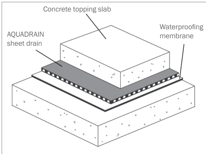
SPLIT-SLAB CONSTRUCTION
